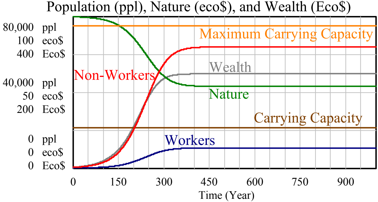
Figure 12: The full collapse that happened in the previous scenario, figure 11, can be prevented by reducing the average depletion per capita. This can be achieved by either increasing the ratio of the Non-Working population or decreasing the average workload per worker, i.e., decreasing total work hours per week.
