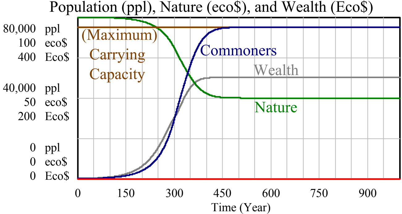
Figure 4: Soft landing to the optimal equilibrium when Elite population (marked in red) equals zero.
