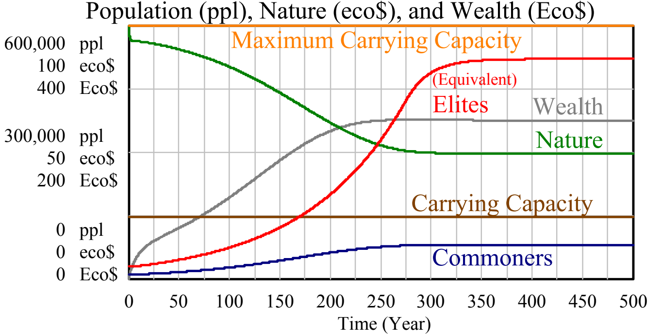
Figure 15: With moderate inequality ( \kappa = 10 ), it is possible to attain an optimal equilibrium by controlling the birth rates.
