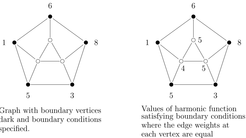
Figure 5.6: Graph illustrating an harmonic function.
