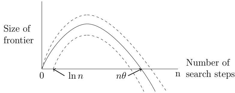
Figure 4.9: The solid curve is the expected size of the frontier. The two dashed curves indicate the high-probability range of possible values for the actual size of the frontier.
