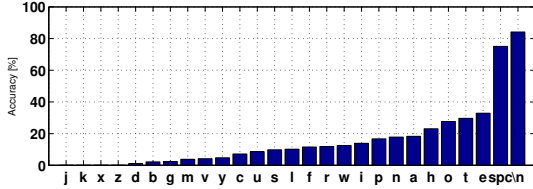
Fig. 4. The accuracy of the keystroke inference per character.
