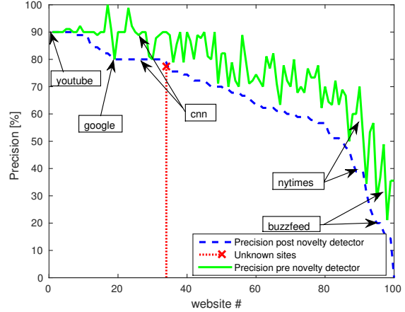
Fig. 8. Novelty detector and classifier combined
